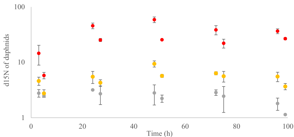
Fig. 3 Evolution of ratios ^{15}\text{N}/^{14}\text{N} ( \delta^{15}\text{N} ) in daphnids without toxicant (control: gray circles) and in daphnids exposed to ^{15}\text{N} tamoxifen via medium (5 \mu\text{g/L} , yellow circles, and 50 \mu\text{g/L} , red circles) and the dietary route. Error bars show standard deviations
