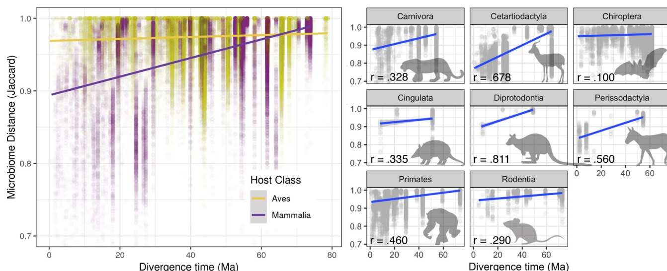
FIG 5 Mammals and birds show different patterns of phyllosymbiosis. (Left) Within host orders, mammals show a generally strong correlation between host distance (estimated divergence time) and microbial community distance (Jaccard), but birds do not. (Right) Within mammalian orders with large sample size, bats (Chiroptera) show the weakest level of phyllosymbiosis. For plots per bird order, see Fig. S7 in the supplemental material.
